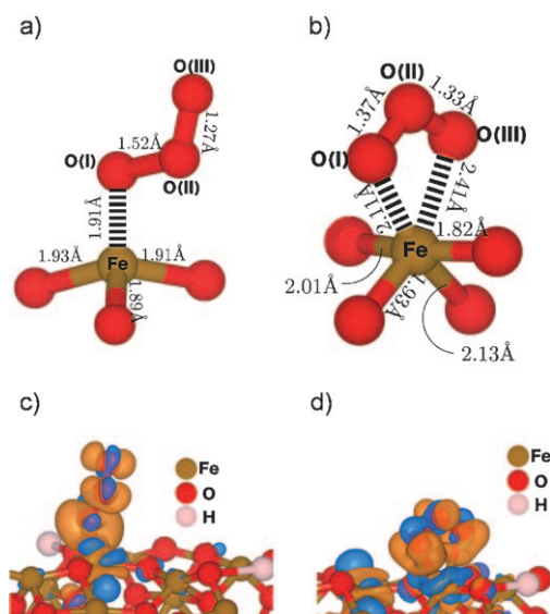
Figure 4. a) The partial structure derived from the optimized structure of O 3 adsorbed on Fh(110) tricoordinated Fe site. b) The partial structure derived from the optimized structure of O 3 adsorbed on Fh(110) tetracoordinated iron site. c, d) Charge density difference \Delta\rho(\mathbf{r}) = \rho_{\text{O}_3/\text{Fh}}(\mathbf{r}) - \rho_{\text{O}_3}(\mathbf{r}) - \rho_{\text{Fh}}(\mathbf{r}) for O 3 adsorbed on Fh(110), where \rho is the charge density and \mathbf{r} denotes the position vector. The charge flows from blue regions to orange regions. c) O 3 adsorbed on Fh(110) tricoordinated iron site, and d) O 3 adsorbed on Fh(110) tetracoordinated iron site.
